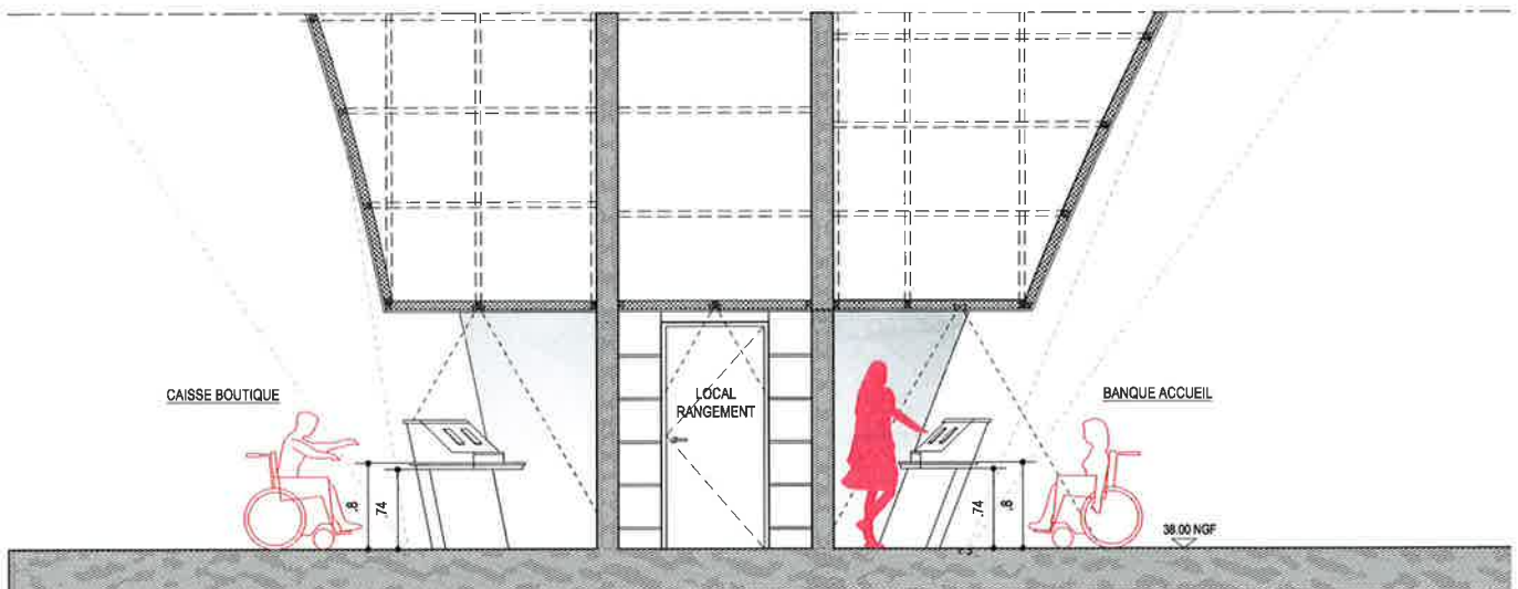
COUPE 2-2'
